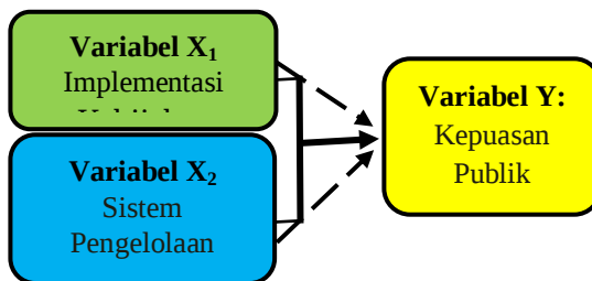
Gambar 1 Model Hipotesis
